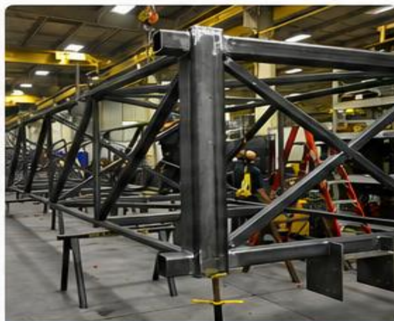
HEAVY FRAME FABRICATION
